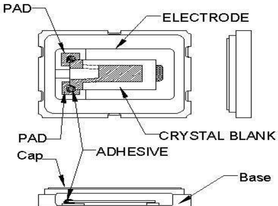
Reference drawing
