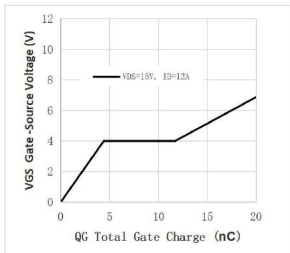
Fig.1 Gate-Charge Characteristics
