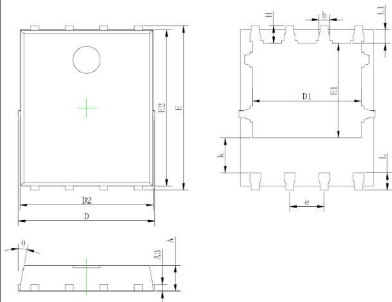
8-Lead DFN5×6 Plastic Package
