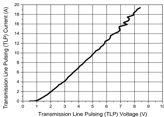
Fig. 6. Ground to Any I/O TLP Curve
