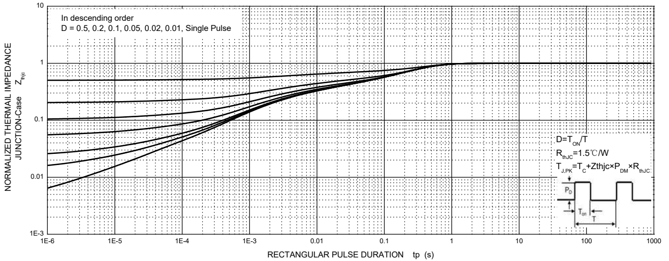
MUR15H60 Transient Thermal Impedance, Junction-Case
