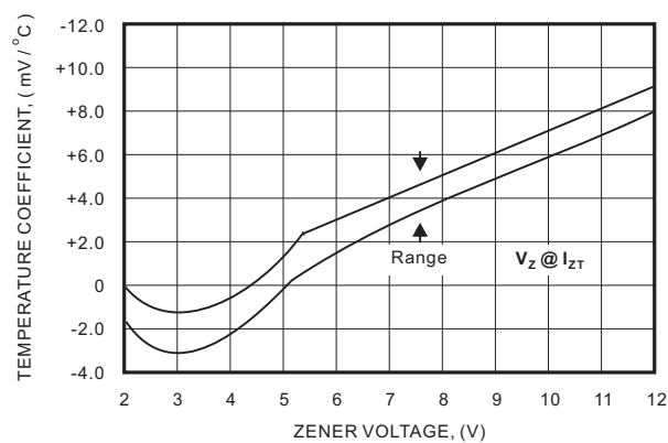
FIG.2A Range for Units to 12 Volts
