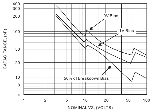
Fig 5. Capacitance Curve
