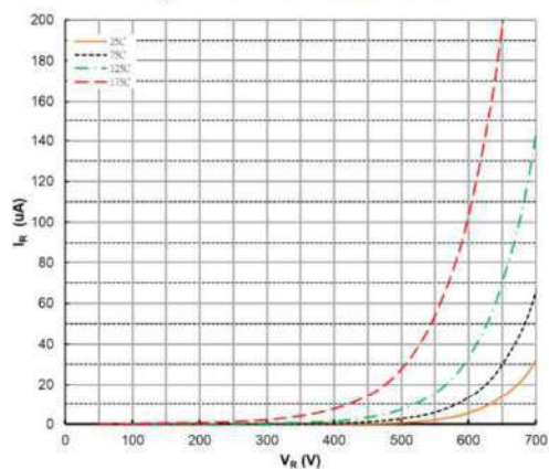
Figure 3. Reverse Characteristics
