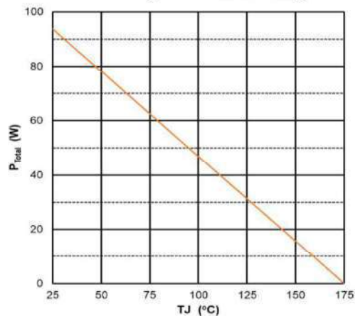
Figure 4. Power Derating
