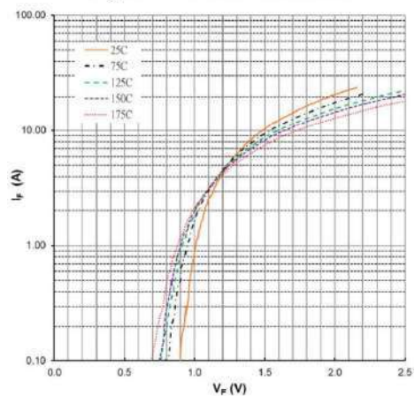
Figure 2. Forward Characteristics
