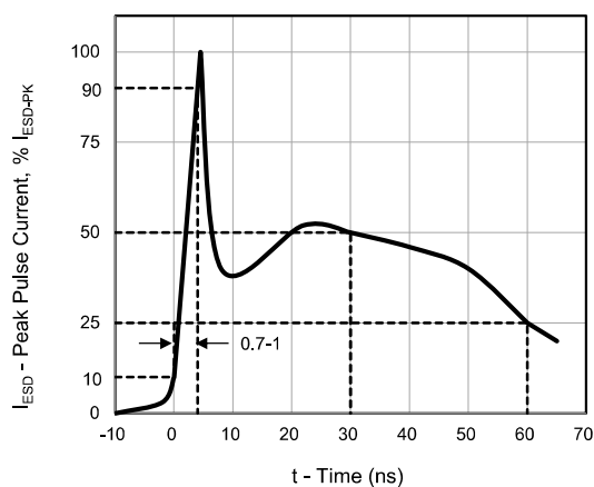
Fig.5 - ESD Pulse Waveform (IEC61000-4-2)
