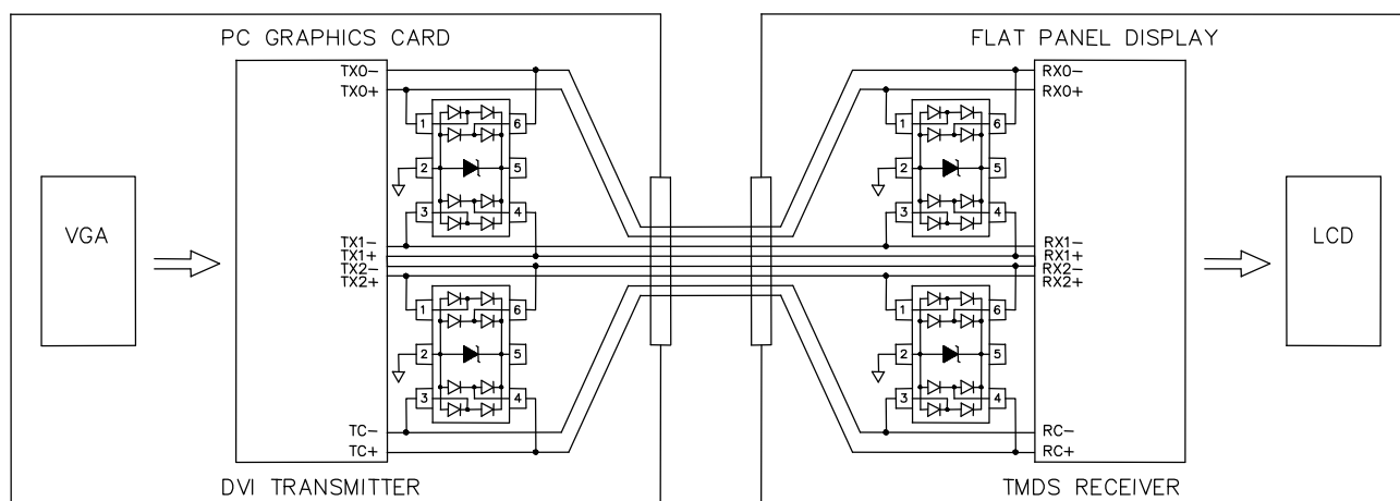
Figure 7 . Digital Video Interface (DVI) Protection
