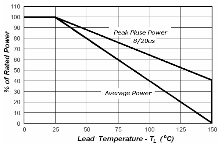
Fig2. Power Derating
