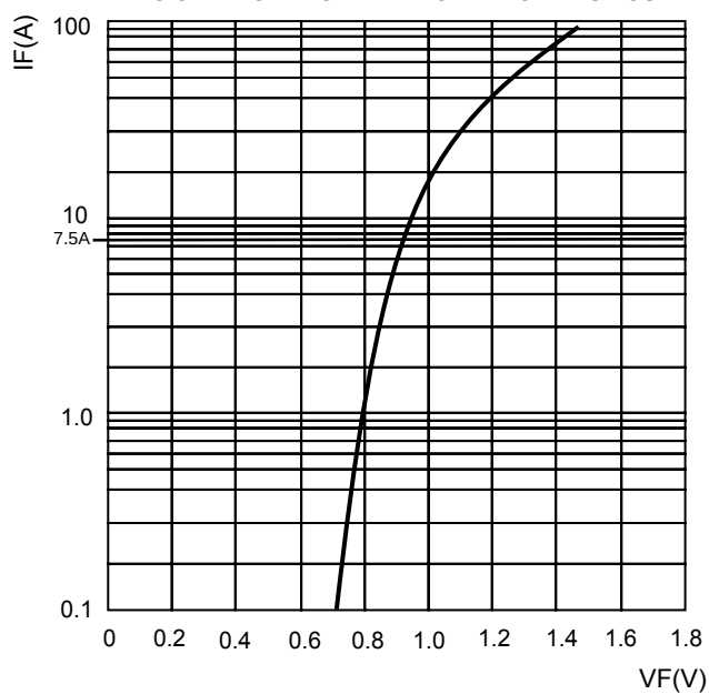
FIG.3-TYPICAL FORWARD CHARACTERISTICS
