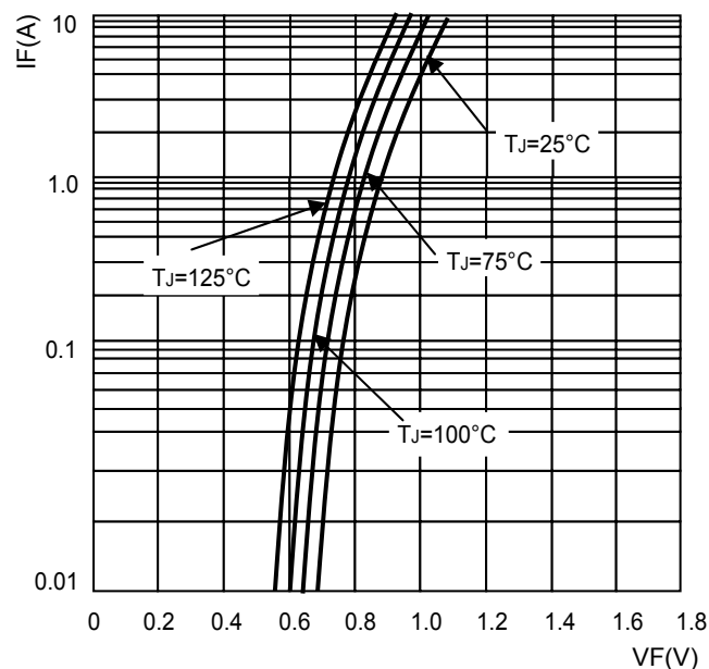
FIG.4-TYPICAL FORWARD CHARACTERISTICS
