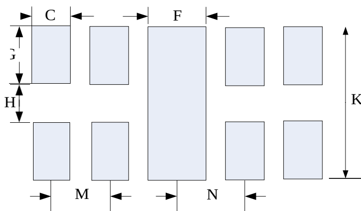
Recommended Solder Pad Footprint
