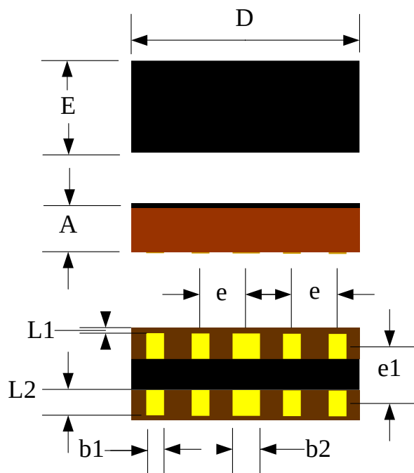
Package outline
