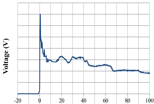
IEC61000-4-2 Pulse Waveform
