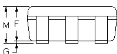
6-Lead TSOP-6 Plastic Surface Mounted Package
