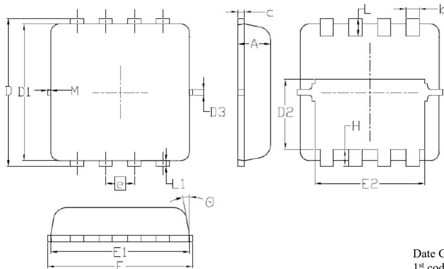
8-Lead DFN3x3 Plastic Package
