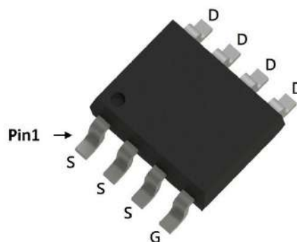
SOP-8
