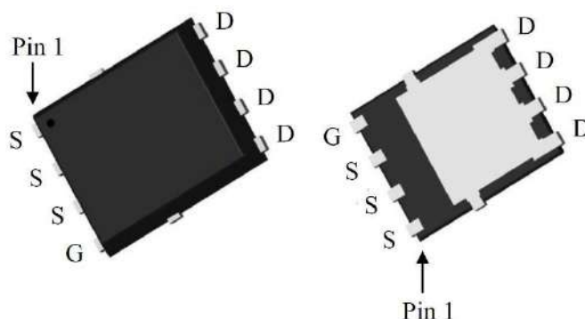
DFN5×6
