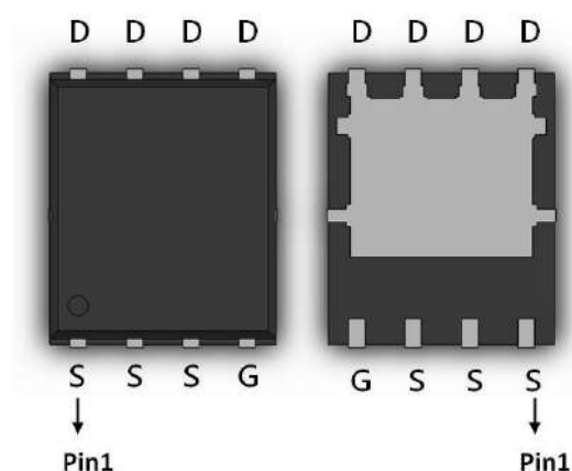
DFN5×6
