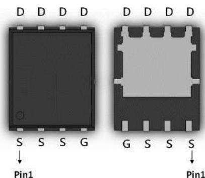
DFN5×6
