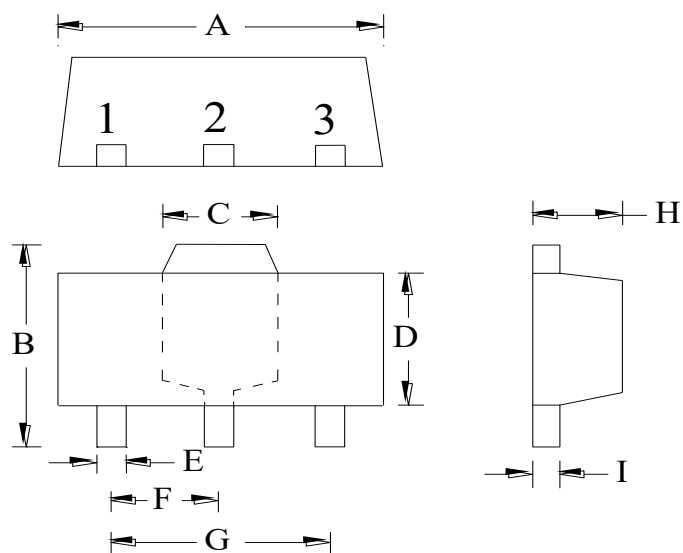
3-Lead SOT-89 Plastic Surface Mounted Package
