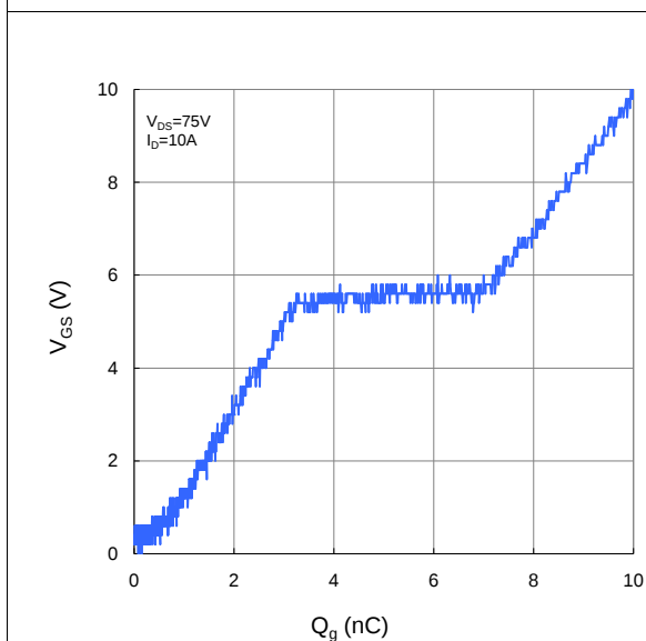
Figure 7. Typical Gate-Charge vs. Gate-to-Source Voltage
