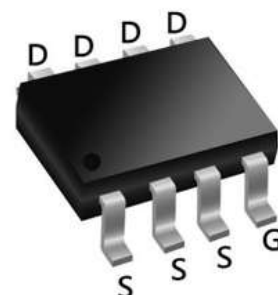
SOP8 Pin Configuration
