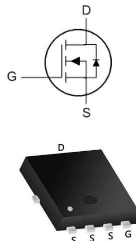
PRPAK5X6 Pin Configuration
