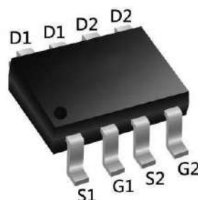
SOP8 Pin Configuration
