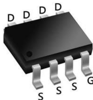
SOP8 Pin Configuration
