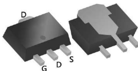
SOT89 Pin Configuration
