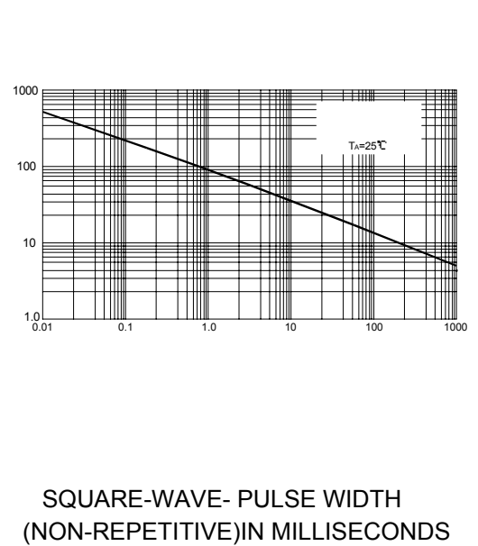
FIG.2 -- TRANSIENT SURGE CAPABILITY
