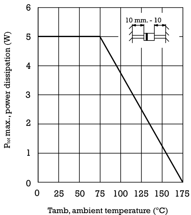
THERMAL RESISTANCE
